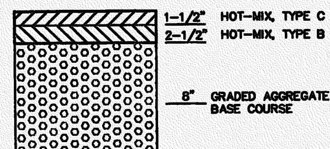
TYPICAL PAVEMENT SECTION NO SCALE
