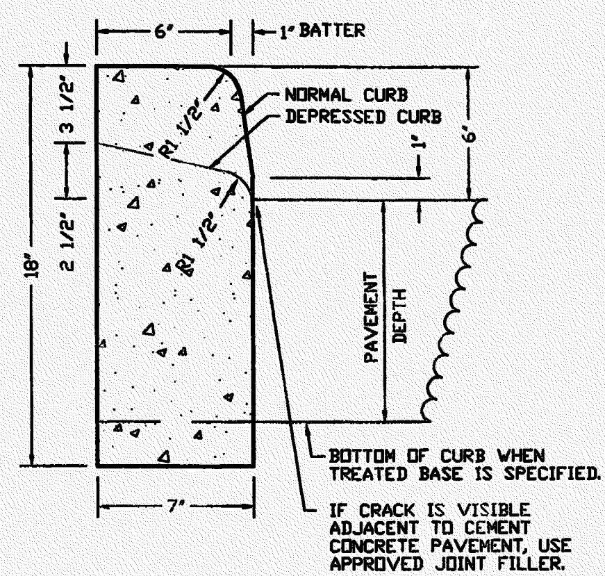
TYPICAL PAVEMENT SECTION NO SCALE
